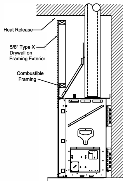
Section View
