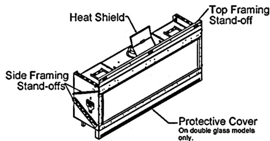
Zero-Clearance Stand-Offs (Isometric View)
