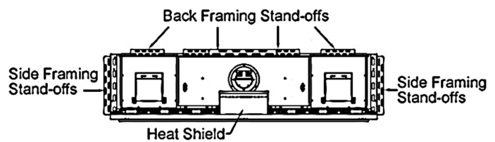
Zero-Clearance Stand-Offs (Top View)
