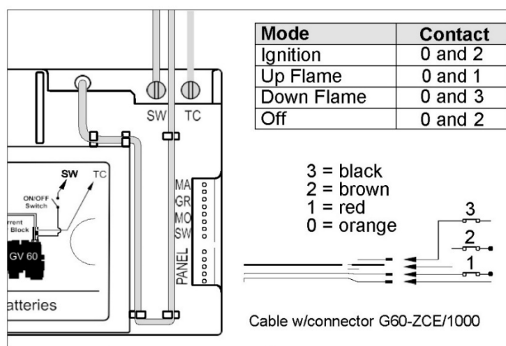
Wiring Diagram and Operation Sequence
