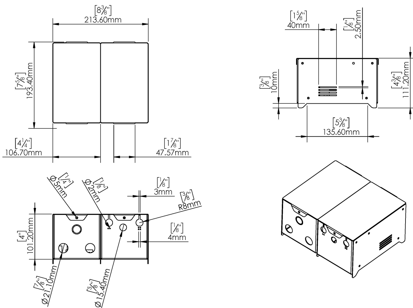
Dimensions for Power Vent Control Box
