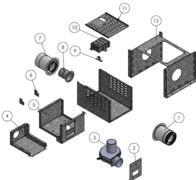
Inline-180 Power Vent Fan Box Components
