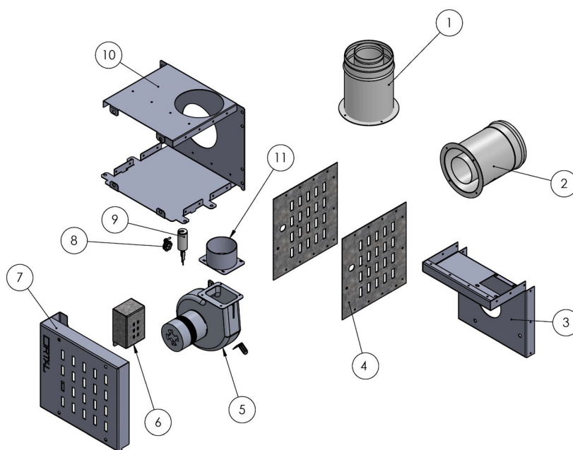
Inline-90 Power Vent Fan Box Components
