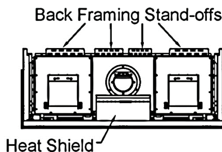
Zero-Clearance Stand-Offs (Top View)
