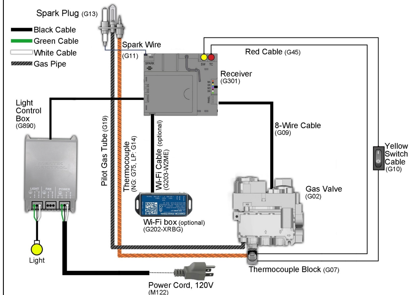
Wiring Diagram: Screen Fireplace with Interior Lighting
